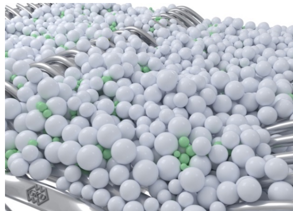
Picture 2: At FILTECH, GKD presents Porometric 25 µm for water filtration as the latest product of this mesh family, which is unparalleled in its ratio of pore aperture to permeability.
