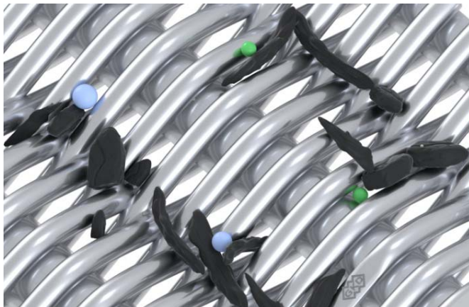
Picture 3: The innovative mesh type ODW6 can be used in all common disc filtration systems. The pore aperture of 6 µm qualifies this mesh for the fight against microplastic.
