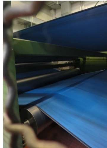
Picture 2: The endless belt of GKD is 30.5 metre long and 4.5 metre wide.
