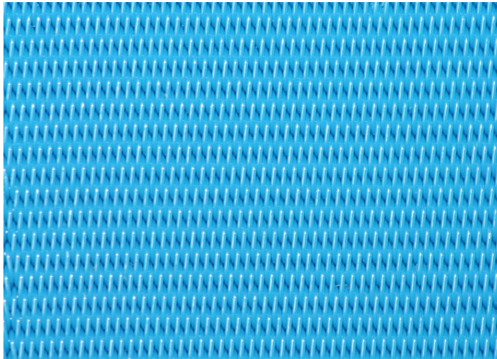
Picture 5: The VACUBELT® 2015 filter belt from GKD is currently setting new standards in lithium dewatering in vacuum drum filters.
