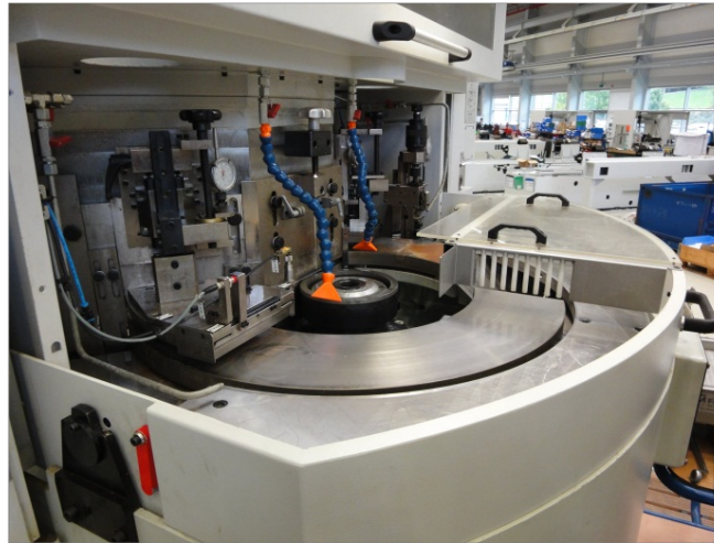
Picture 5: The Supfina double disk grinding Planet series makes a convincing case with great reliability.
