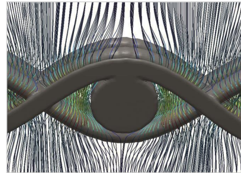
Picture 6: CFD-simulation of an Optimized Dutch Weave made by GKD.
