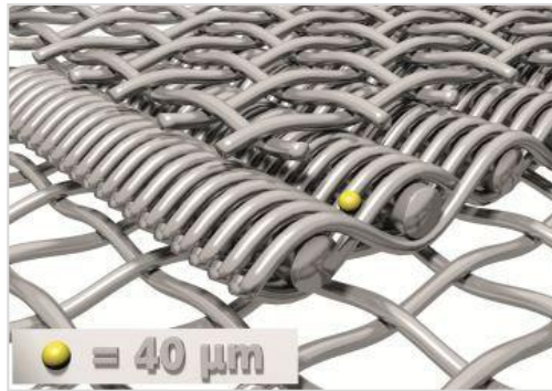
Picture 5: The optimised plain dutch weaves by GKD have a pore size from 10 to 50 µm.
