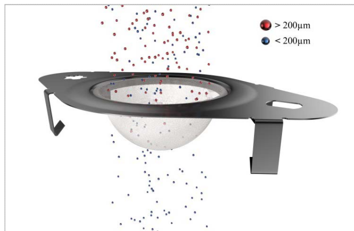
Picture 3: The constructed component filtered reliably out all particles above the size of 200 µm before the EGR low pressure loop.
