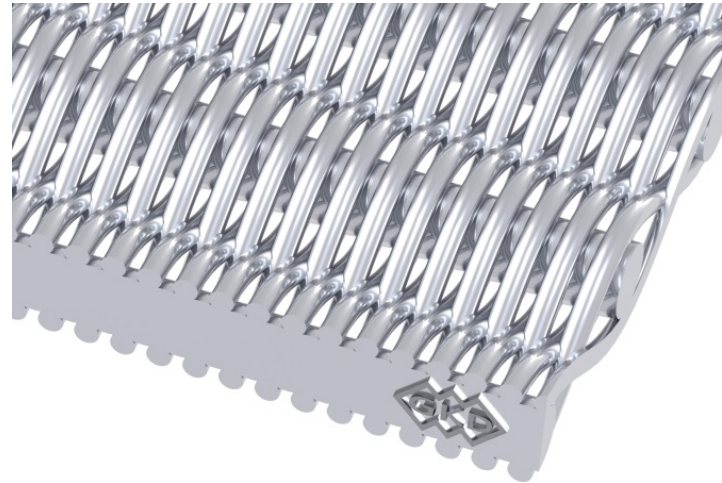
Picture 2: Optimized dutch weaves from GKD are characterized by significantly more and finer weft than warp wires.
