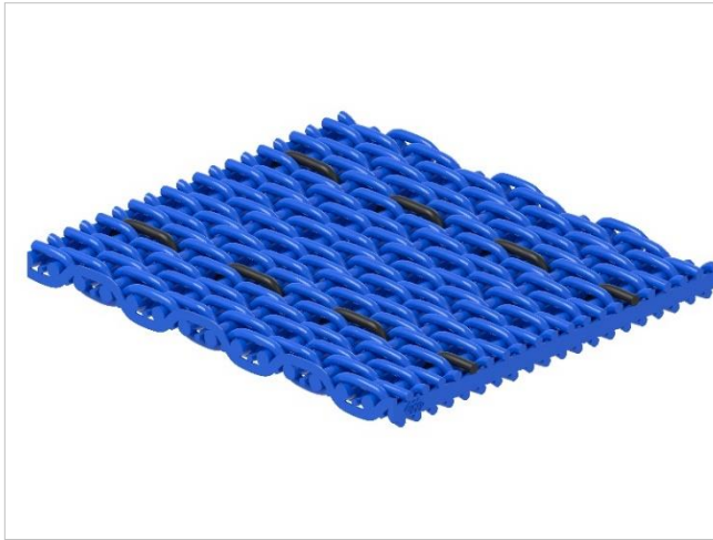
Picture 1: Thanks to the special topography of its belt surface, the new CONDUCTIVE 2215 process belt fabric from GKD guarantees precise deposit without fiber entanglement or fiber loss during nonwoven forming with airlay and meltblown processes.
